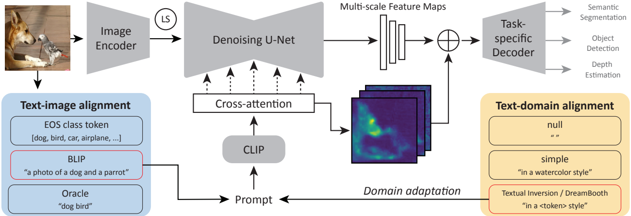
Figure 2. Overview of TADP. We encode images using the latent scaling (LS) described in Sec. 4.1. We experiment with several prompting strategies and evaluate their impact on downstream vision task performance. Our method concatenates the cross-attention maps and the multi-scale feature maps before passing them to the vision-specific decoder. In the blue box, we show three single-domain captioning strategies with differing levels of text-image alignment. We propose using BLIP [24] captioning to improve image-text alignment. We extend our analysis to the cross-domain setting (yellow box), exploring whether aligning the source domain text captions to the target domain may impact model performance by appending caption modifiers to image captions generated in the source domain and find model personalization modifiers (Textual Inversion/Dreambooth) work best.
